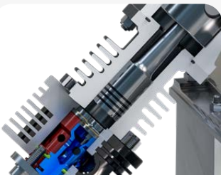
Second, third and fourth stage with pushing pistons to eliminate lateral forces on the pistons
