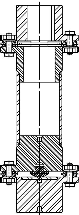
SXV Type for Vertical Mounting
