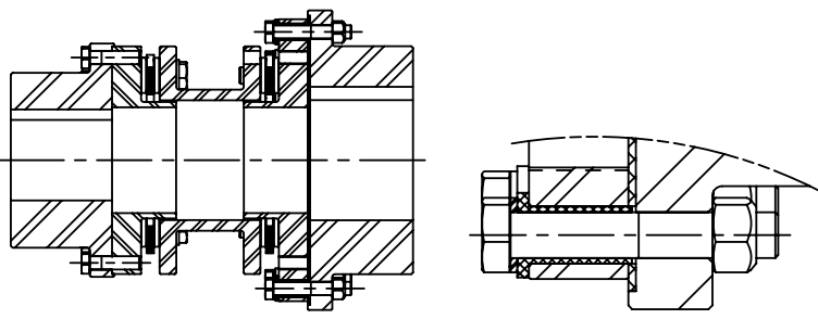
DIEI Type with Electrical Insulation
