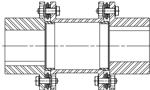
SXLEF Type with LEF Limited End Float
