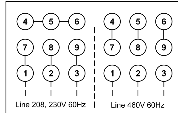
Figure 5.25 EP.NA - WYE
