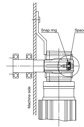
Figure 5.5 Secured by Spacer and Snap Ring
