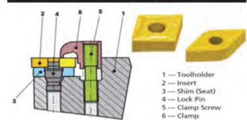
Combination Pin & Clamp "M" System
